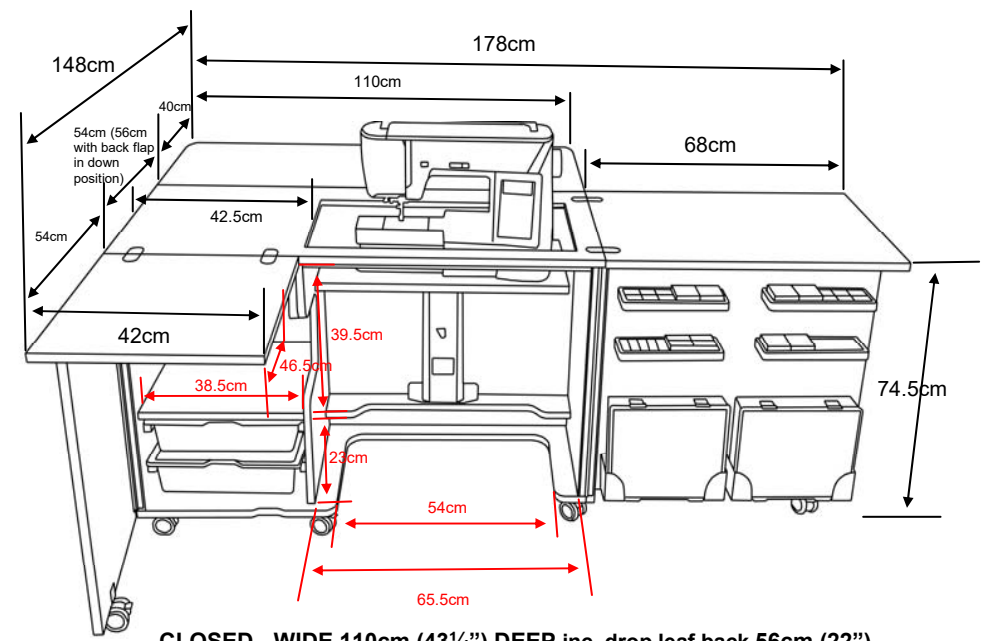
CLOSED - WIDE 110cm (43 1/4") DEEP inc. drop leaf back 56cm (22") HIGH 76cm (30")
