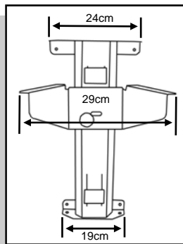
Front dimensions
